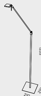
P-76 1 x LED 5W 500lm 3000K ⏻-⏻
