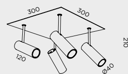
PL-43 4 x LED 5W 500lm 3000K
