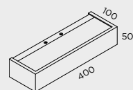
A-811/40 2 x R7s 78mm 80W Max. IP44
