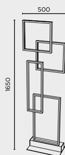
P-194 LED 56W 8960lm 3000K
