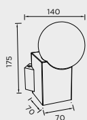
A-176 1 x G9 48W Max. (LED RECOMMENDED)
