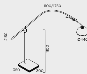
P-127 1 x E-27 60W Max.
