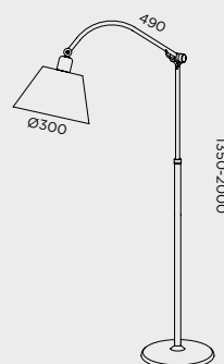
P-1005 1 x E-27 60W Max.
