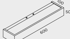
A-811/60 3 x R7s 78mm 80W Max. IP44
