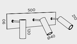
A-42 3 x LED 5W 500lm 3000K
