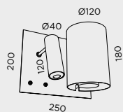
A-133 E-27 PL + LED 5W 500lm 3000K ON-ØFF x 2
