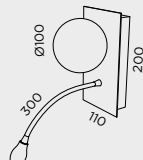
A-136 LED 3W 195lm 3000K + 69 33W/LED
