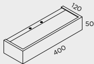
A-811/40 EMERG LED LED 20W 3000lm 3000K
