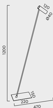
P-45 1 x LED 5W 500lm 3000K
