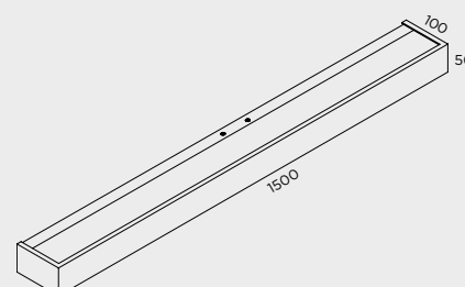
A-812/150 LED 82W 12420lm 3000K DIMMABLE
