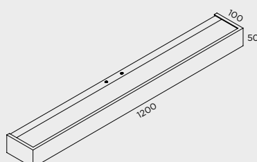
A-812/120 LED 65W 9920lm 3000K DIMMABLE
