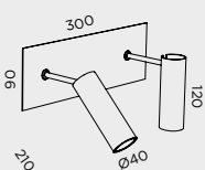
A-41 2 x LED 5W 500lm 3000K
