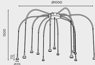
C-198/13 LED 39W 2535lm 3000K
