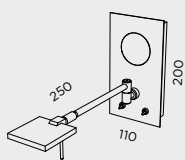
A-134 LED 5W 500lm 3000K + LED 8W 900lm 3000K ON-ØFF x 2
