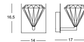
KARAT PA 1 1 x MAX 42W G9 alo. ENERGY SAVER CE F IP 20
