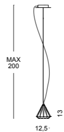
KARAT SO 1 1 x MAX 42W G9 alo. ENERGY SAVER CE F IP 20
