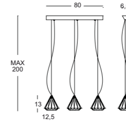
KARAT S3L 3 x MAX 42W G9 alo. ENERGY SAVER CE F IP 20
