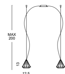
KARAT SO 2 2 x MAX 42W G9 alo. ENERGY SAVER CE F IP 20
