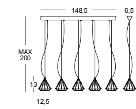
KARAT S5L 5 x MAX 42W G9 alo. ENERGY SAVER CE F IP 20
