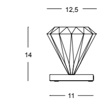
KARAT CO 1 x MAX 42W G9 alo. ENERGY SAVER CE F IP 20
